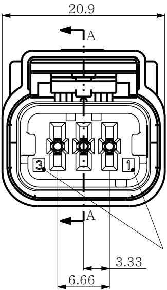
CIRCUIT NO.
