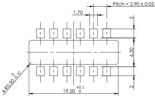
PCB Pattern - SMT
