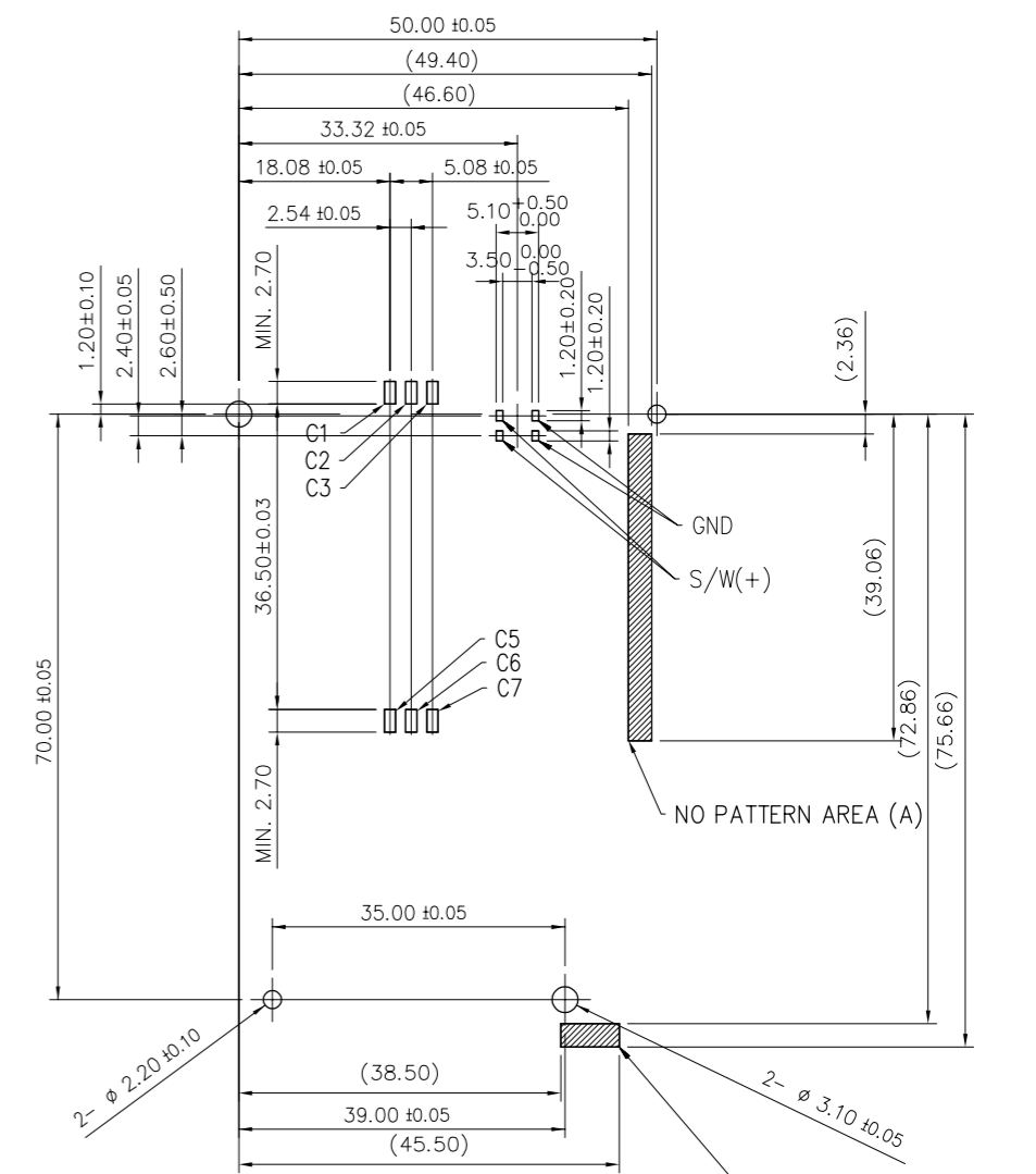
RECOMMENDED P.C.B PATTERN SCALE 1:1
