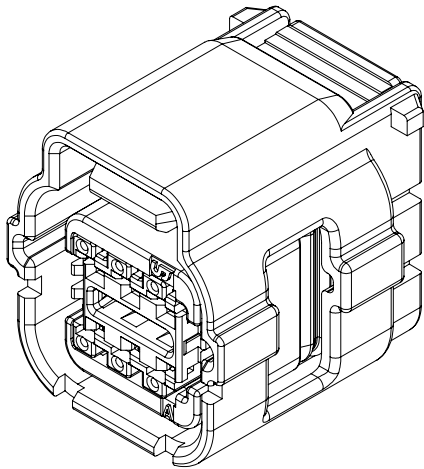
ISO View
